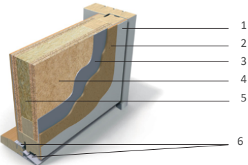
PREMIUM (80mm) 1. Laminat/Maling/Dekor 2. Laminat 3. Aluminiumsplate 4. Isolasjon 5. Ramtre 6. Tettelist 7. Aluminiumsplate 8. Laminat/Maling/Dekor BRANNDØR (62mm) TREND TETT SLETT EI30/35DB 1. Malt ytterside 2. HDF plate 3. Alu fuktsperre 4. Brannhemmende plate 5. Rockwool 6. Alu/tre terskel
