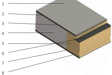
PLUS (60mm) 1. Laminat/Maling/Dekor 2. Laminat 3. Aluminiumsplate 4. Isolasjon 5. Ramtre 6. Tettelist 7. Aluminiumsplate 8. Laminat/Maling/Dekor
