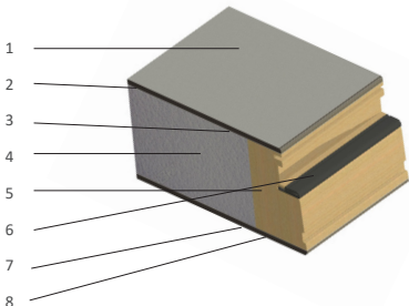
PREMIUM (80mm) 1. Laminat/Maling/Dekor 2. Laminat 3. Aluminiumsplate 4. Isolasjon 5. Ramtre 6. Tettelist 7. Aluminiumsplate 8. Laminat/Maling/Dekor
